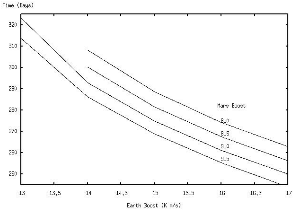
Figure 1. Optimum times.
